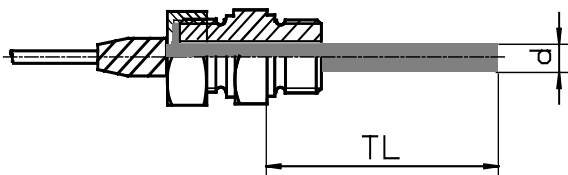
Stem type F6 union nut with rotating thread
