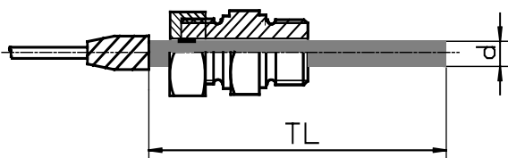
Stem type F7 plain stem, smooth with clamping nut
