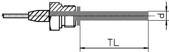
Stem type F5 rotating thread only with extra thermowell
