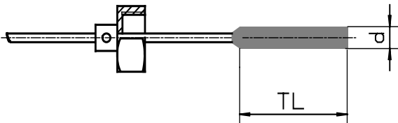
Stem type F4-1 displacable union nut on capillary
