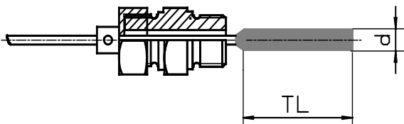
Stem type F7-1 displacable union nut on capillary with clamping nut
